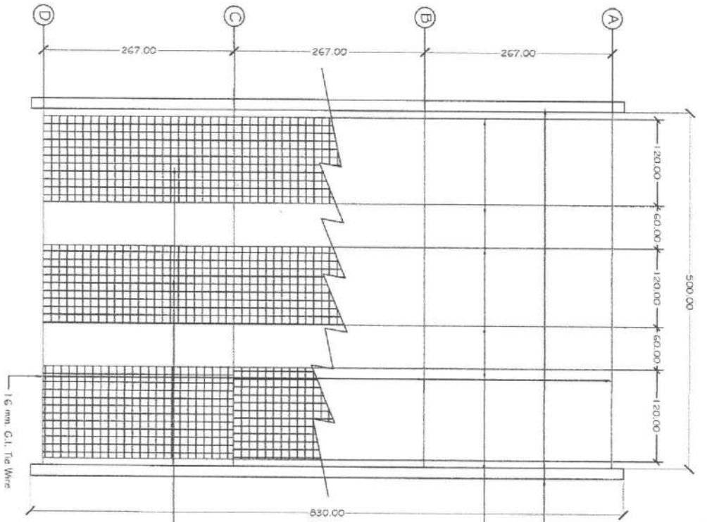
TOP ELEVATION (NET COVERING) SCALE 1:50 MTS
