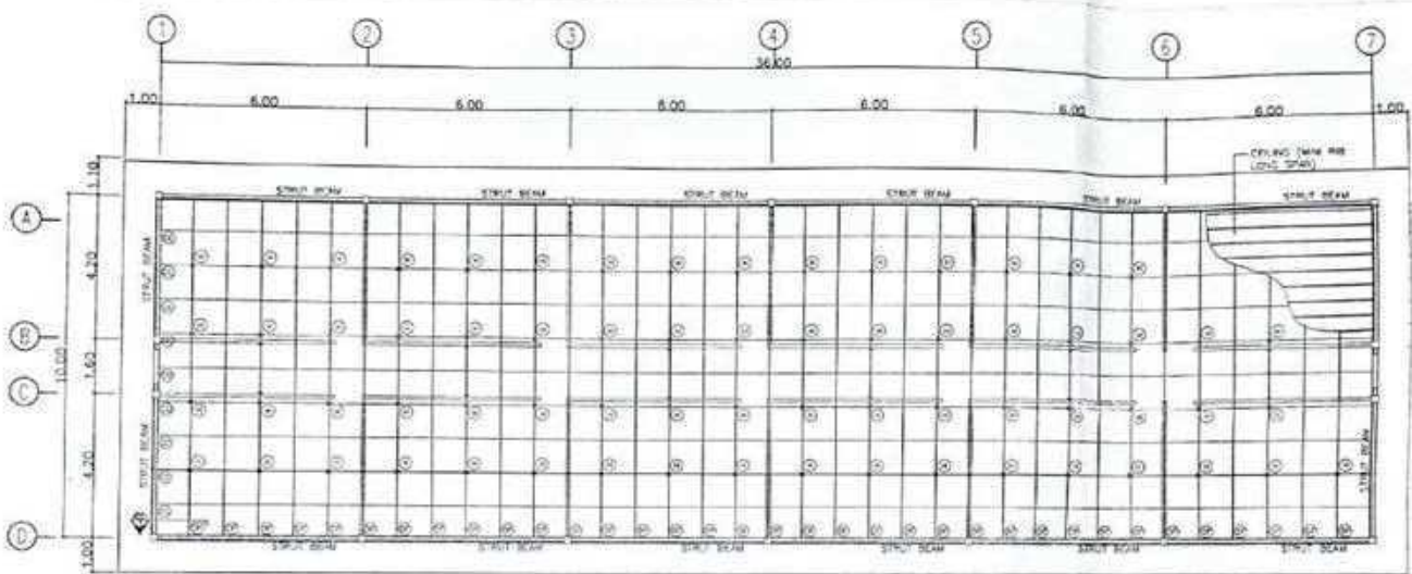
CEILING FRAME DETAIL SCALE: 1/8\"/>
